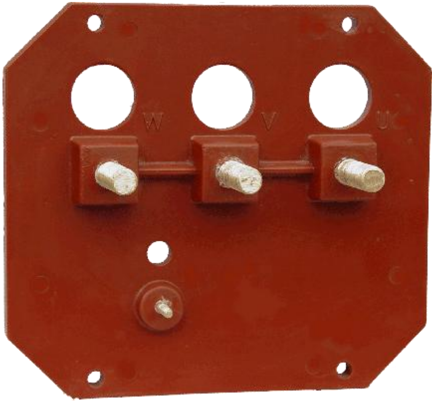
Epoxy Motor Terminal Plate
