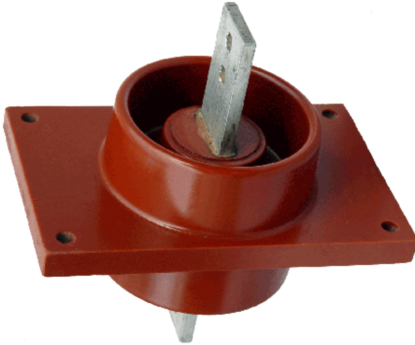
11KV Epoxy Bushing PG-SOB4
